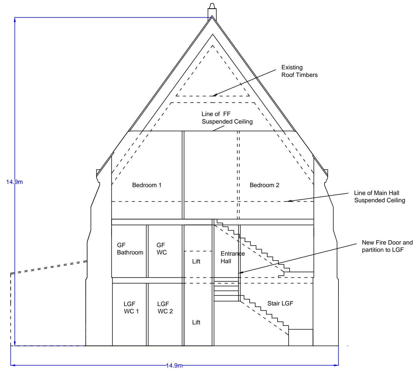
8DT18: 8 Derby Terrace North Section A, As Proposed Page 1 of 1, Scale 1:100 at A3
